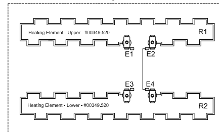
Heating Elements
